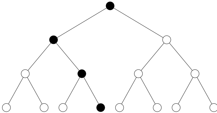
Figure 1: The binary tree used in the construction of the lower bound. The black nodes correspond to a potential sequence.
